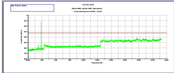
Port 0, 2480 MHz
