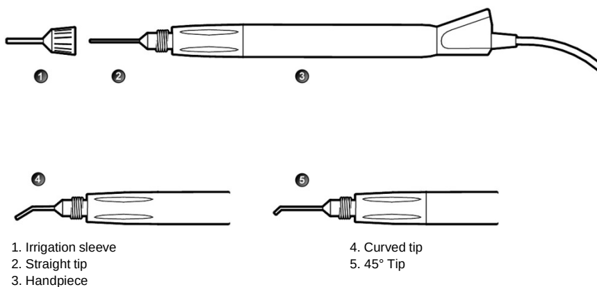
Figure 3.6 – I/A Handpiece Assembly
