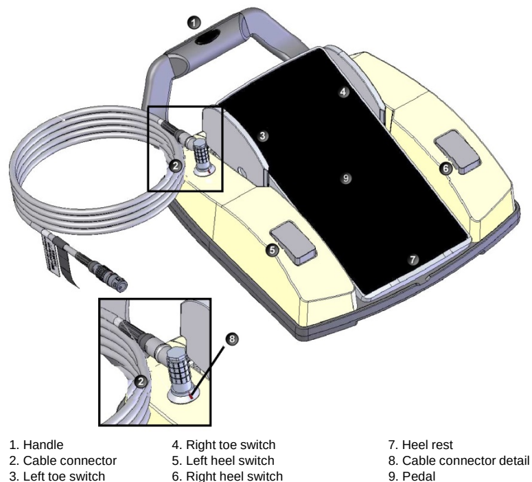
Figure 4.5 – Single Linear Foot Pedal
