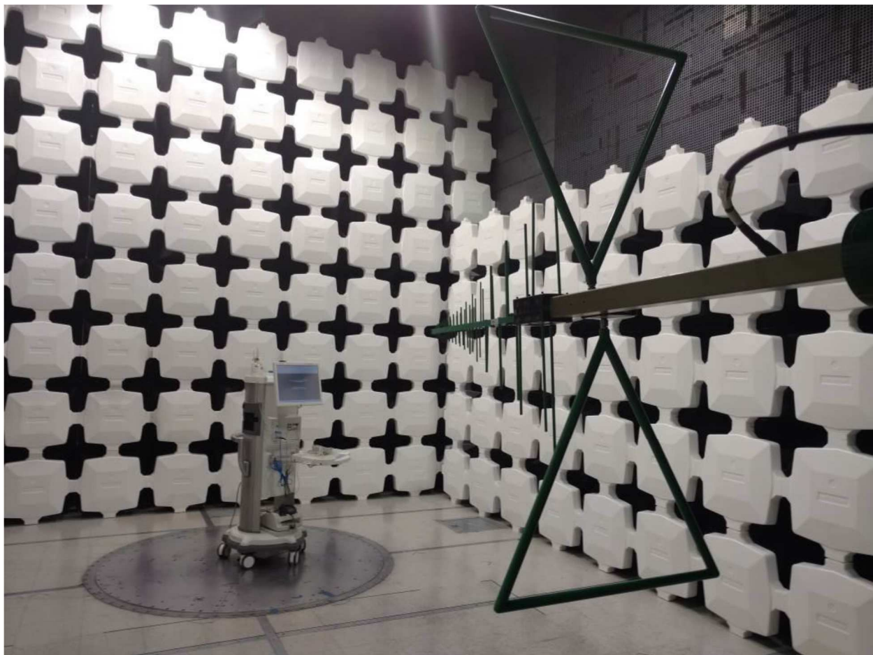
Radiated Measurements 30MHz to 1GHz
