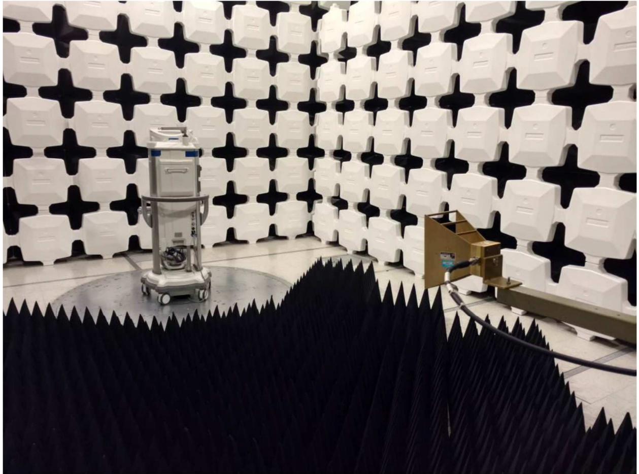
Radiated Measurements above 1GHz
