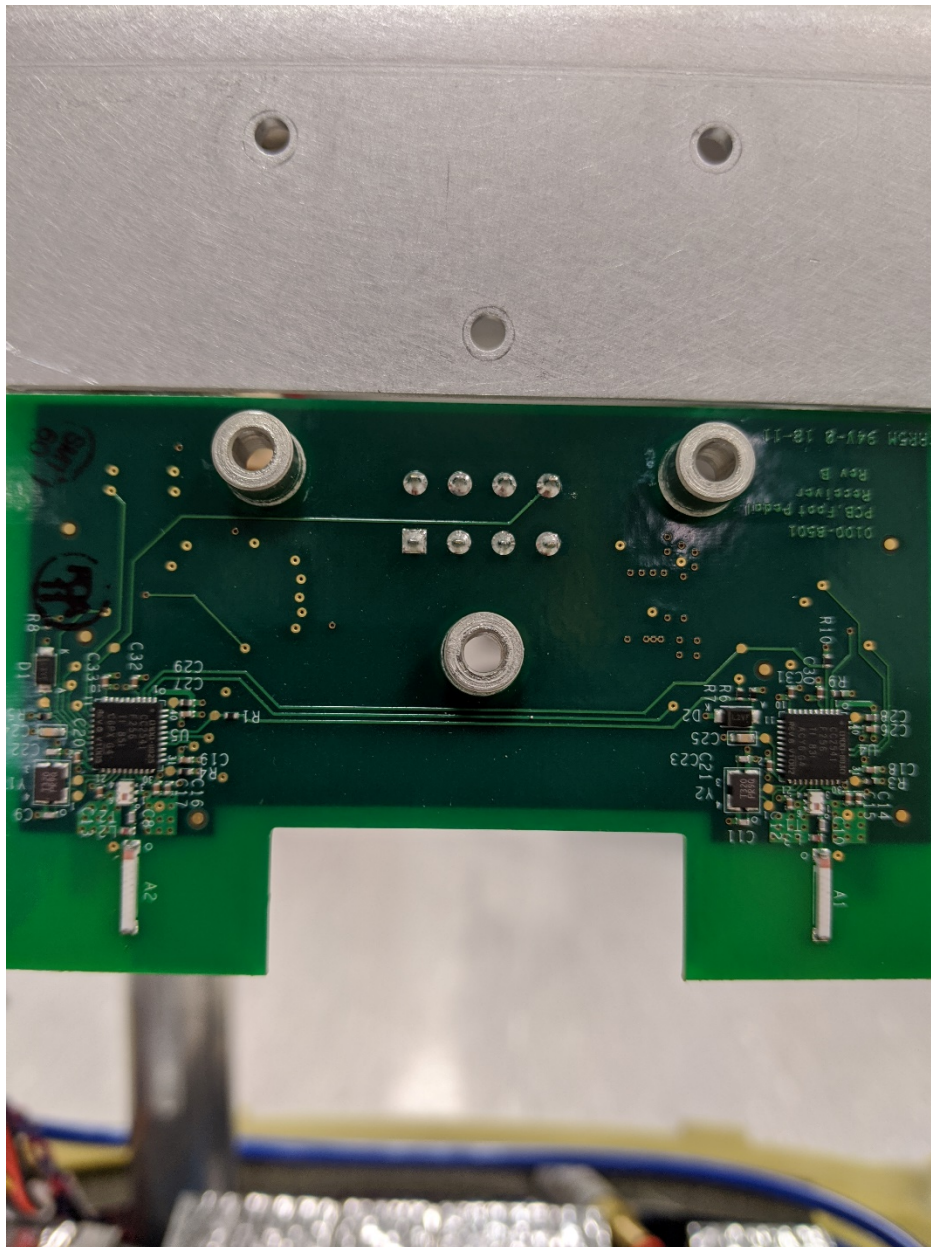
RF module for BLE Foot Pedal control mounted in main system
