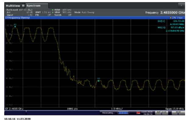
DH5, High Channel
