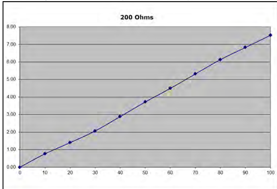
Figure 12-3 — Diathermy Output Power (Typical) 200 Ohm
