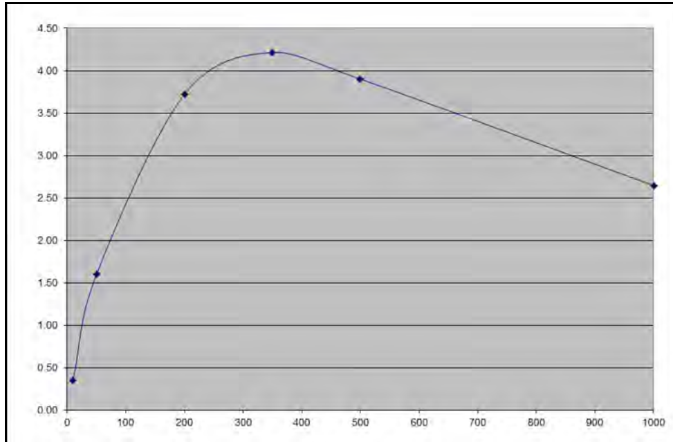
Figure 12-7 — Diathermy Output Power (50% Setting)
