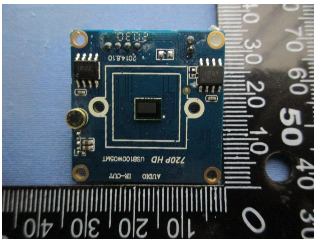
19. Rear view of PCB 5 (Unshielded)
