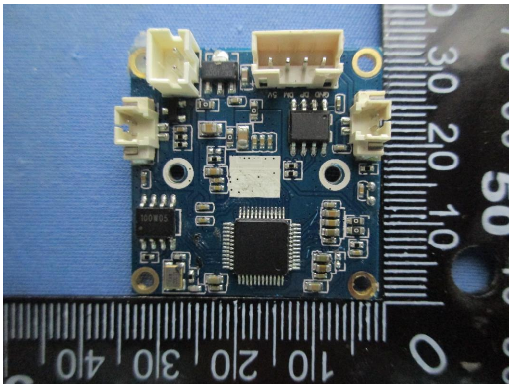
18. Front view of PCB 5 (Unshielded)
