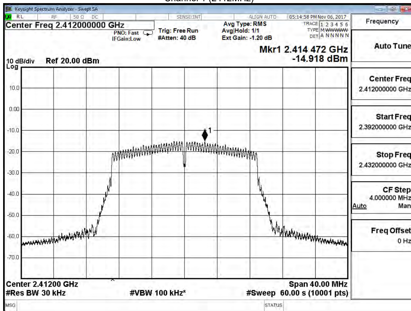
Channel 1 (2412MHz)
