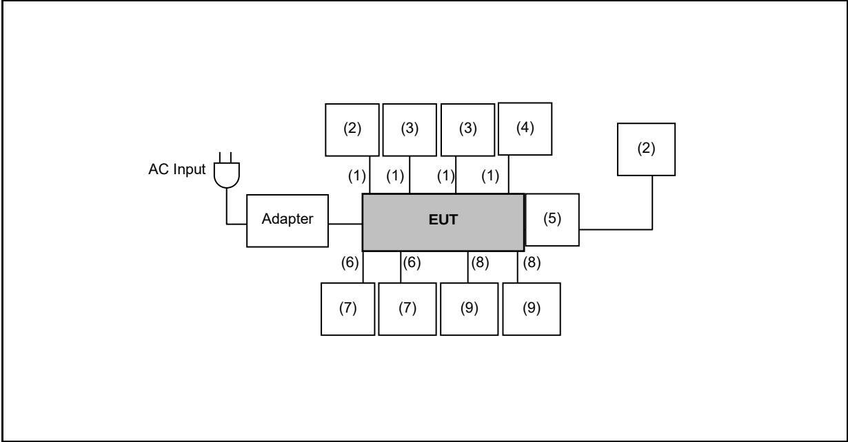
Conducted Emissions
