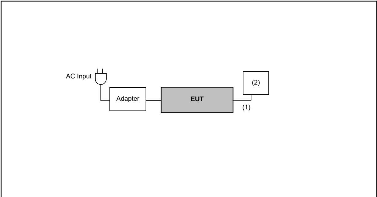
Radiated Emission
