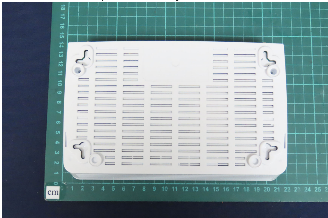
(2) EUT Photo - Trademark: DrayTek, Model No.: Vigor2767Vax
