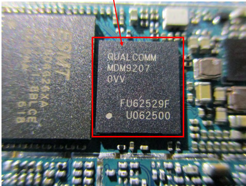
2G/3G/4G/GPS Chip – Top View
