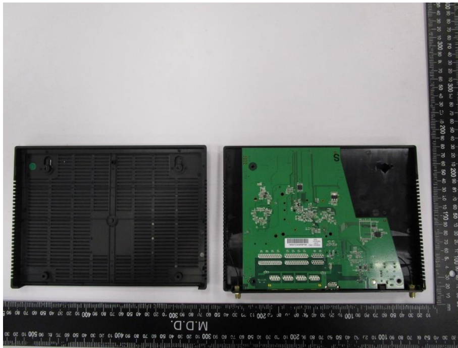
Model : Vigor2915Fac
