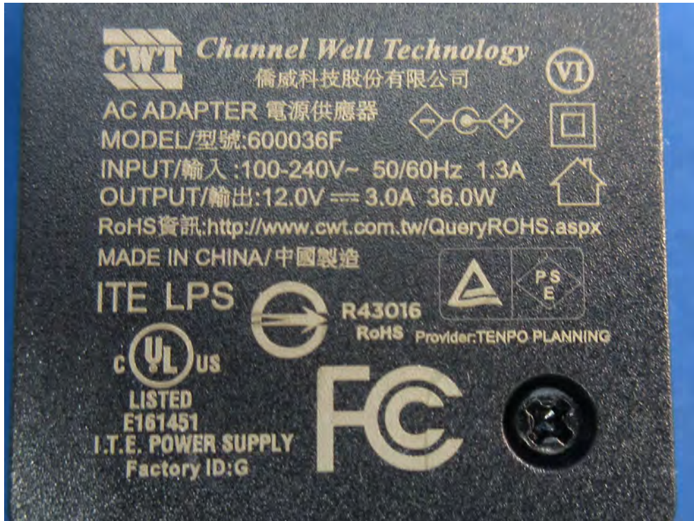
(36) EUT Photo (Adapter 2)
