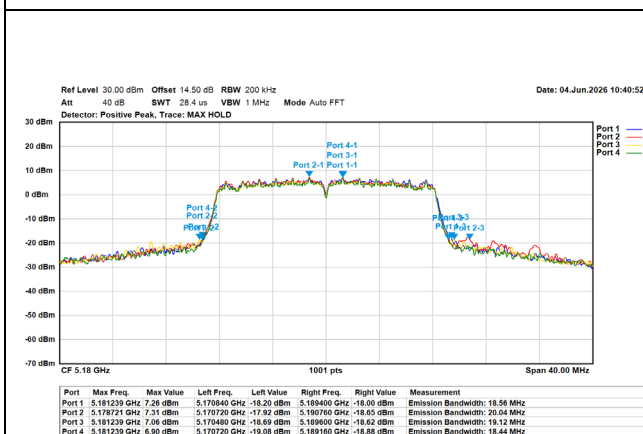
802.11a/20MHz/6M/5180MHz/Ch36
