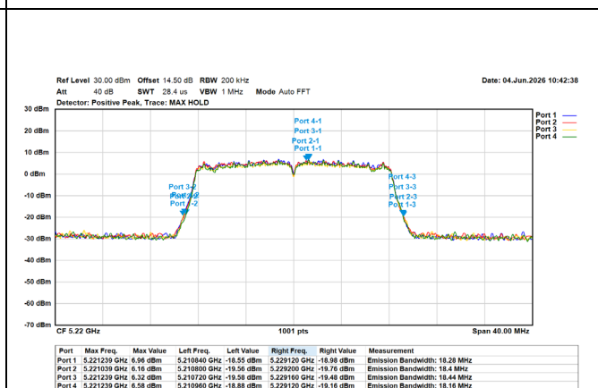
802.11a/20MHz/6M/5220MHz/Ch44
