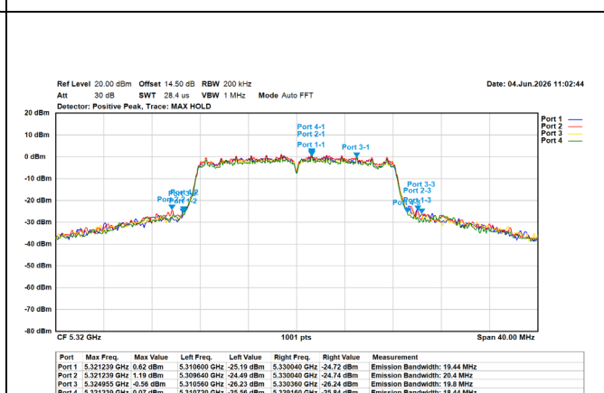
802.11a/20MHz/6M/5320MHz/Ch64
