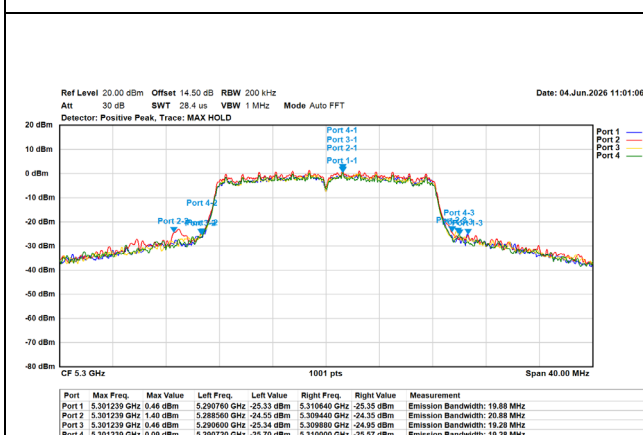
802.11a/20MHz/6M/5300MHz/Ch60
