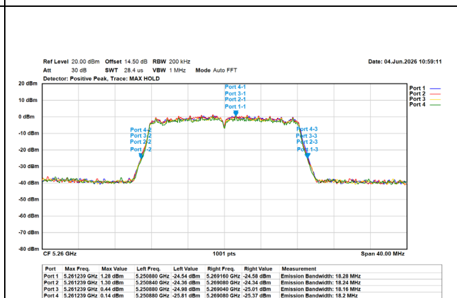
802.11a/20MHz/6M/5260MHz/Ch52
