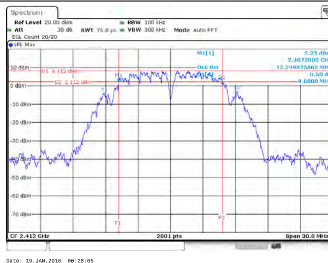
Minimum Emission Bandwidth Plots (6dB)
