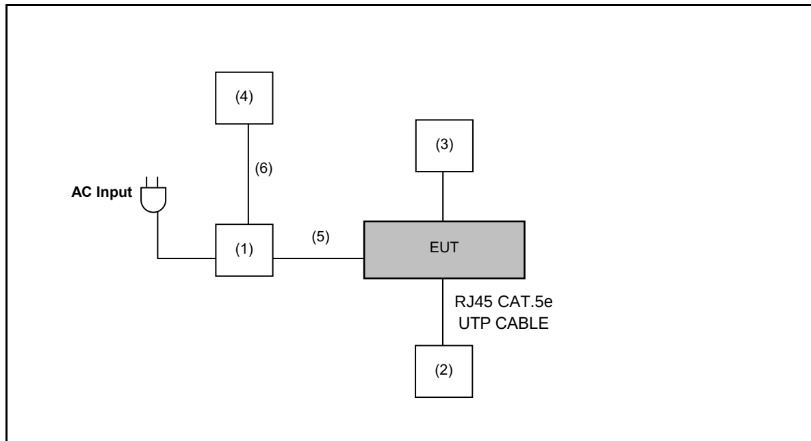
Conducted Emission
