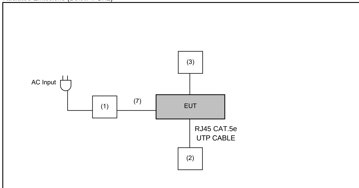
Radiated Emissions (Below 1 GHz)
