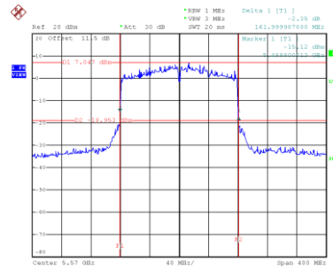
CH114 26 dB Bandwidth
