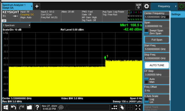
Radar Burst at the End of the Channel Availability Check Time
