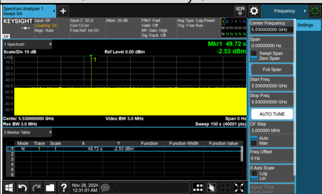
Radar Burst at the Beginning of the Channel Availability Check Time
