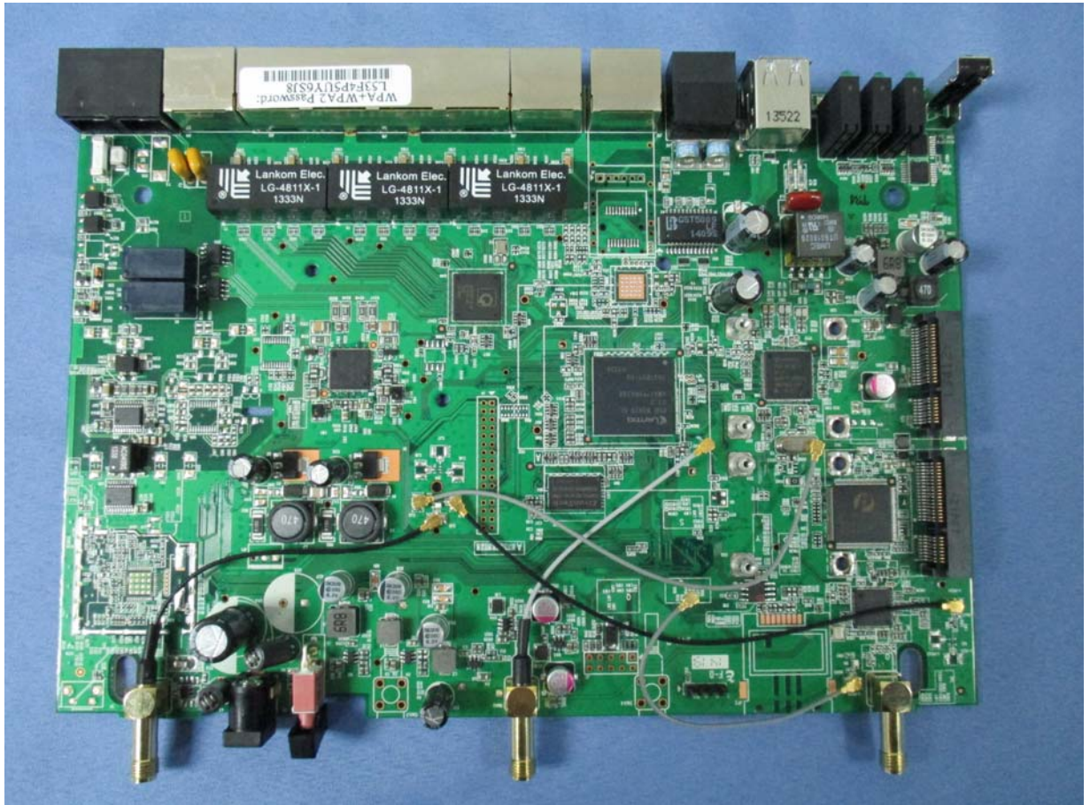
(16) EUT Photo (MB)
