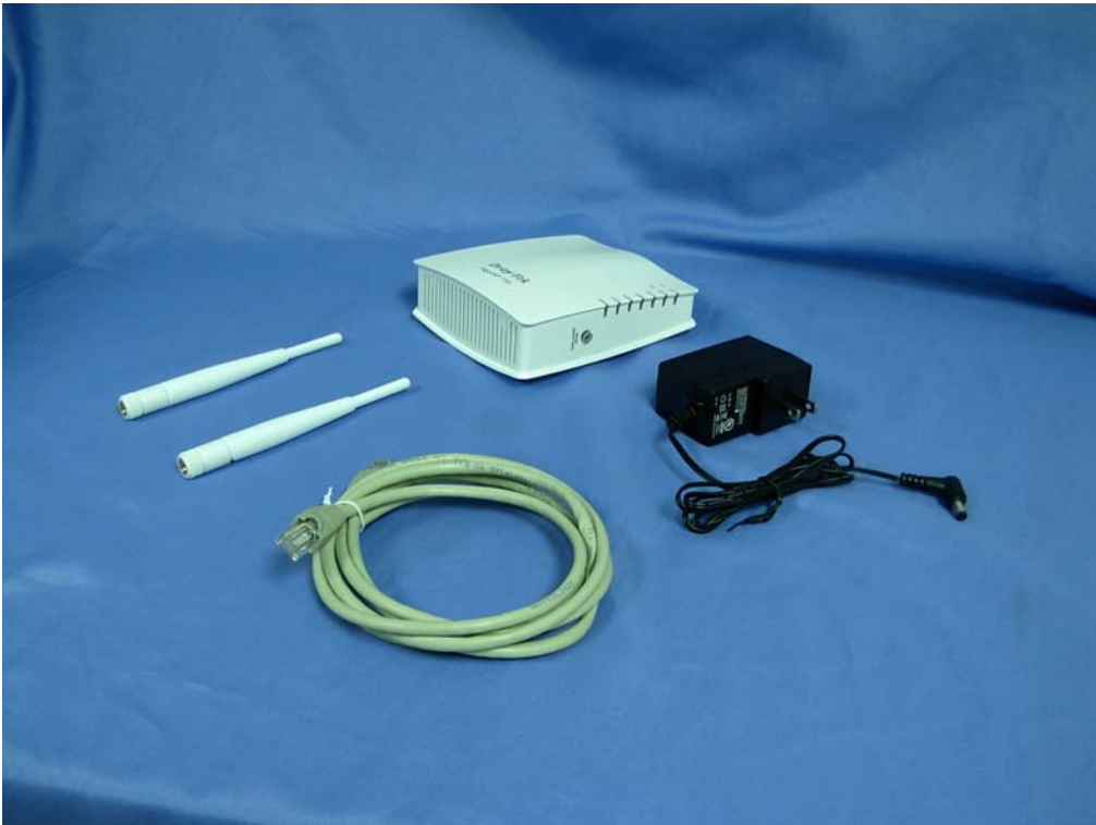
(5) EUT Photo ( Walsin / PI_RFDPA131300SBAB802, EUT: VigorAP710 )
