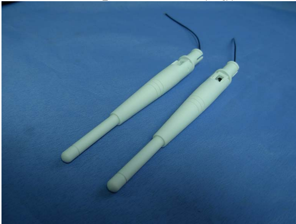
(26) EUT Photo (Antenna: Walsin / PI_RFDPA131307NNAB301(Short), PI_RFDPA131311NNAB301(Long) )
