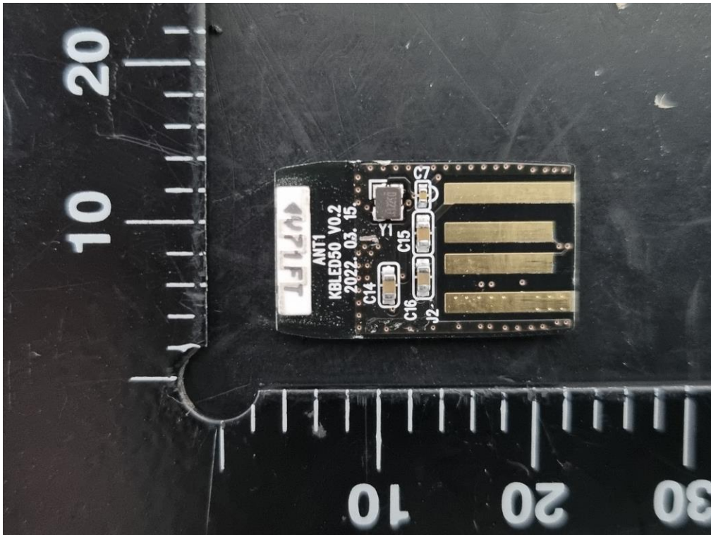
Main Board(Front)
