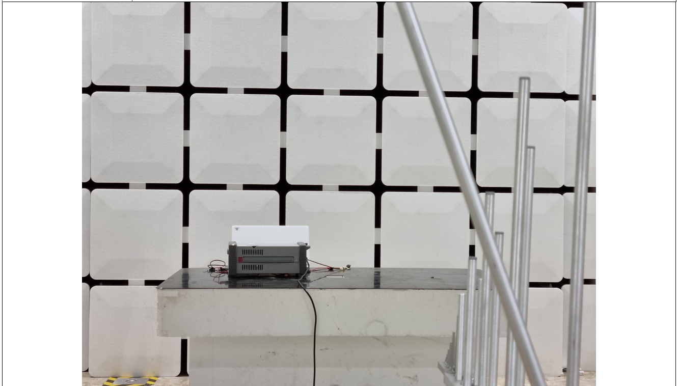
Radiated measurement for below 1 GHz (Rear side)
