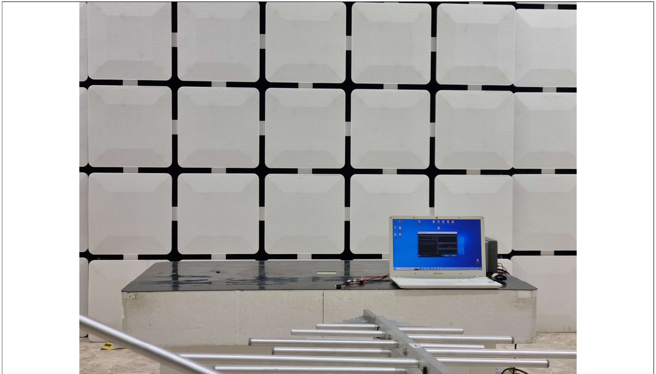
Test Setup
