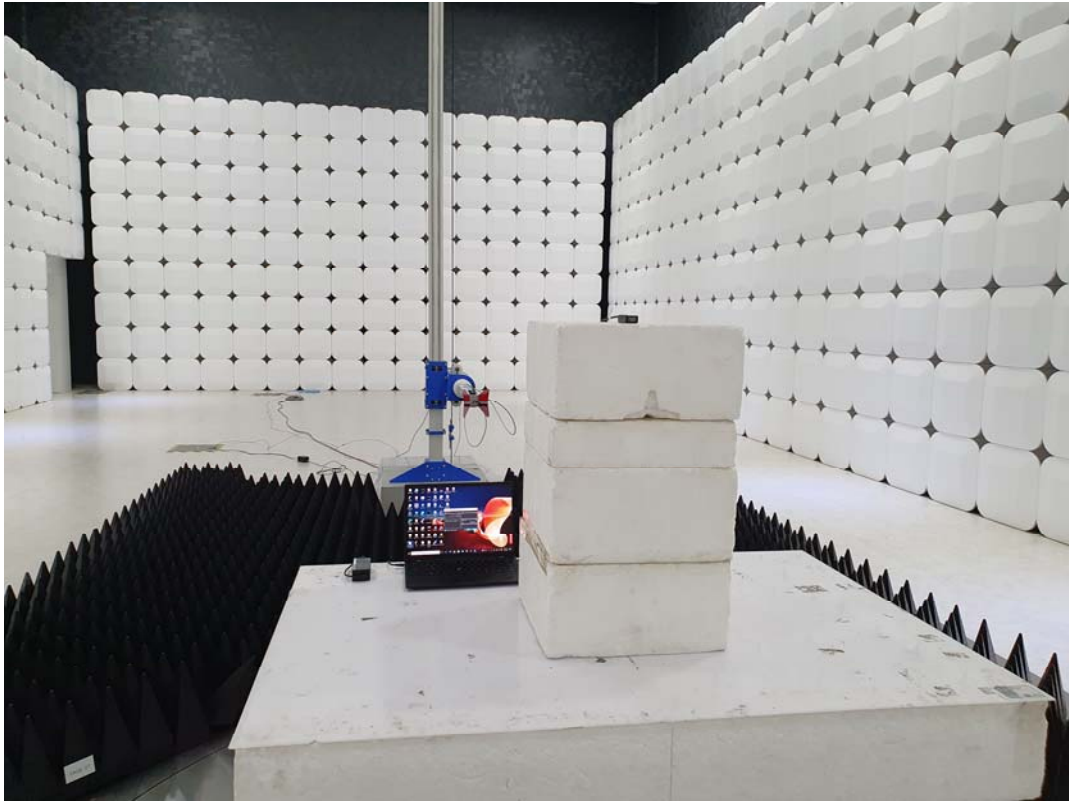
Radiated emission test (1 GHz to 7 GHz)
