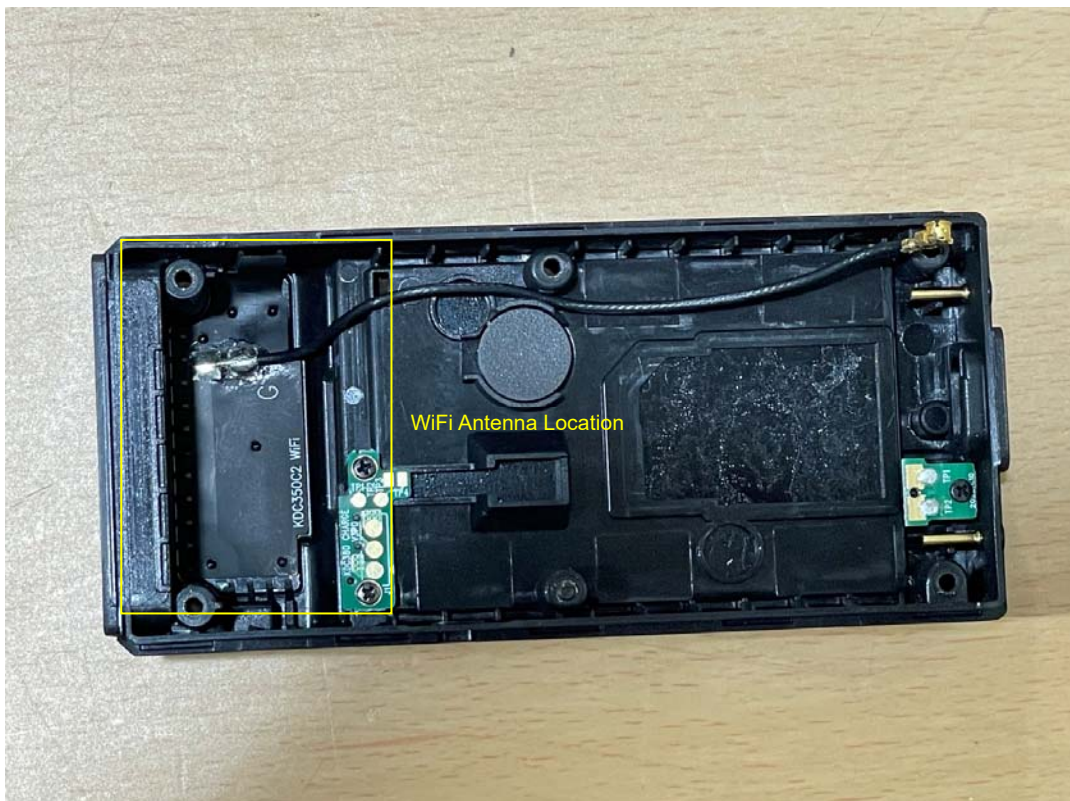
WiFi Antenna
