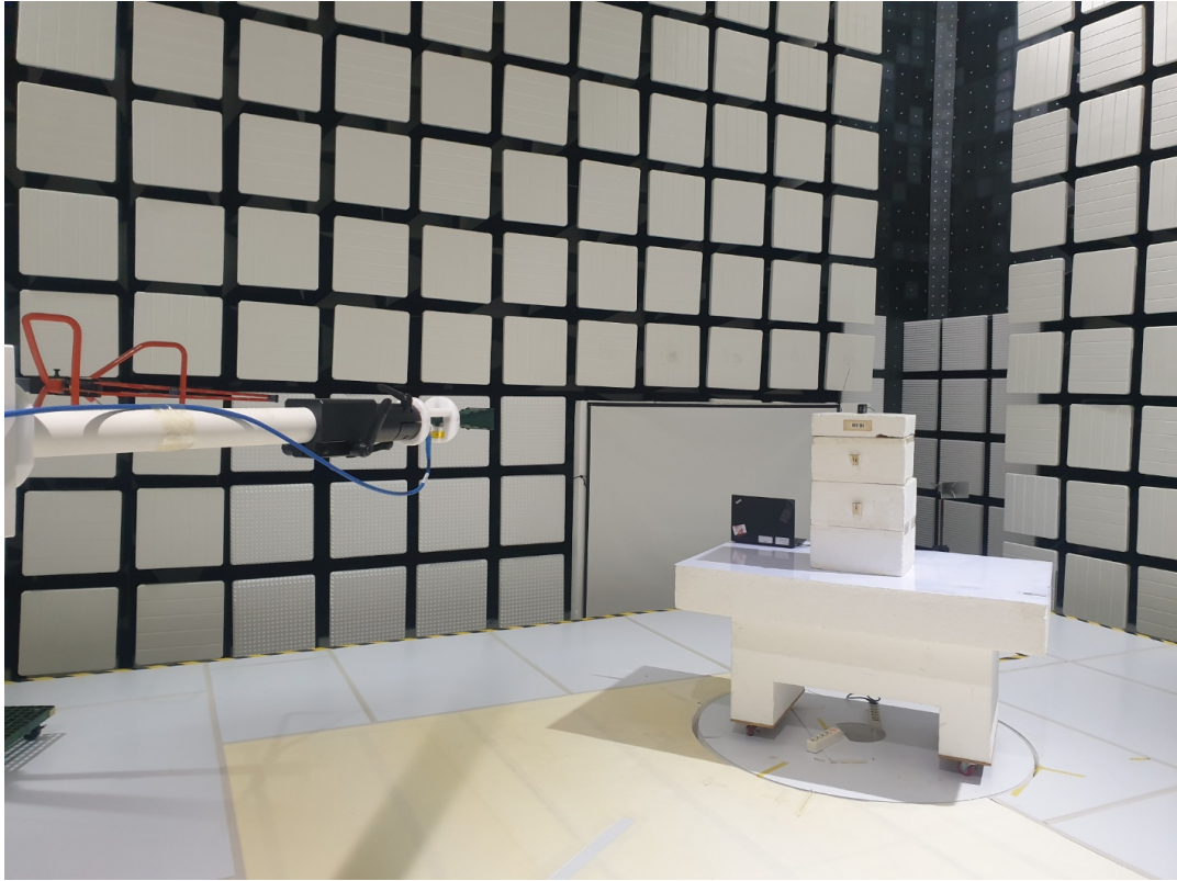
Radiated emission test (18 GHz to 26.5 GHz)
