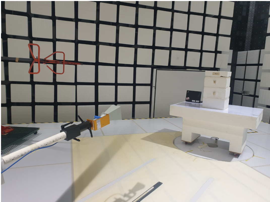
Radiated emission test (6.5 GHz to 18 GHz)
