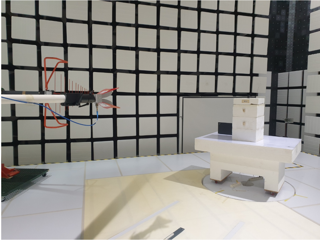
Radiated emission test (1 GHz to 6.5 GHz)
