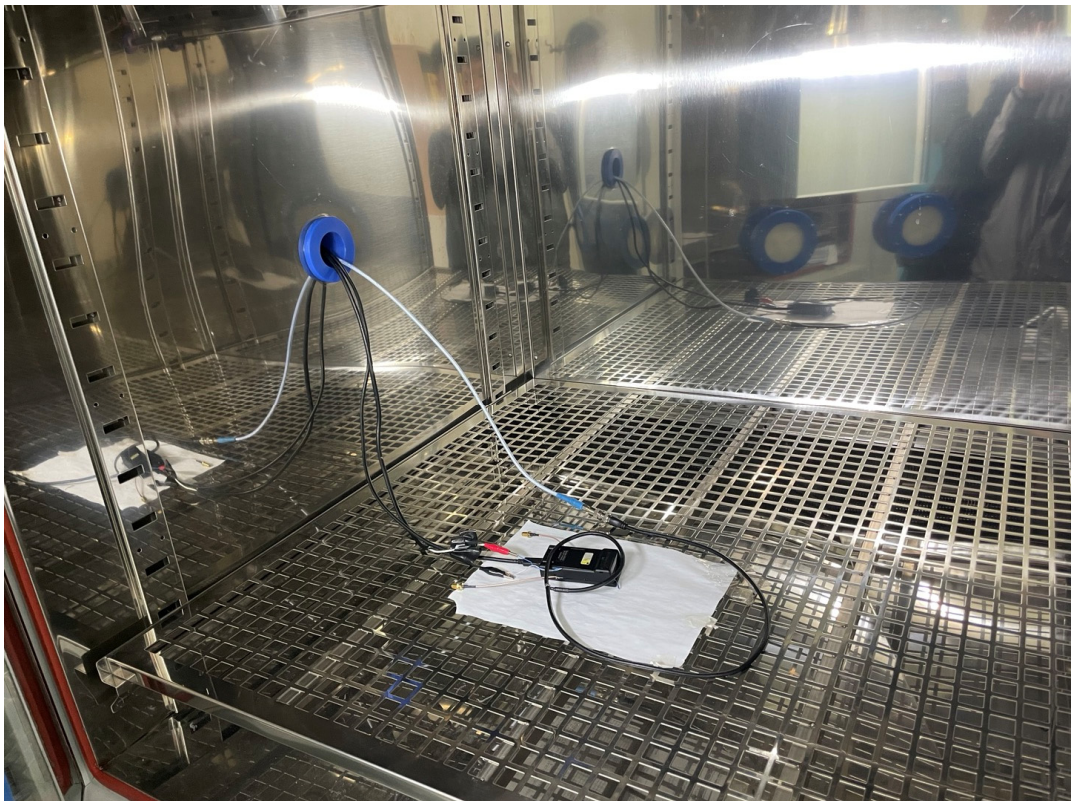
Conducted RF measurements in the temperature chamber
