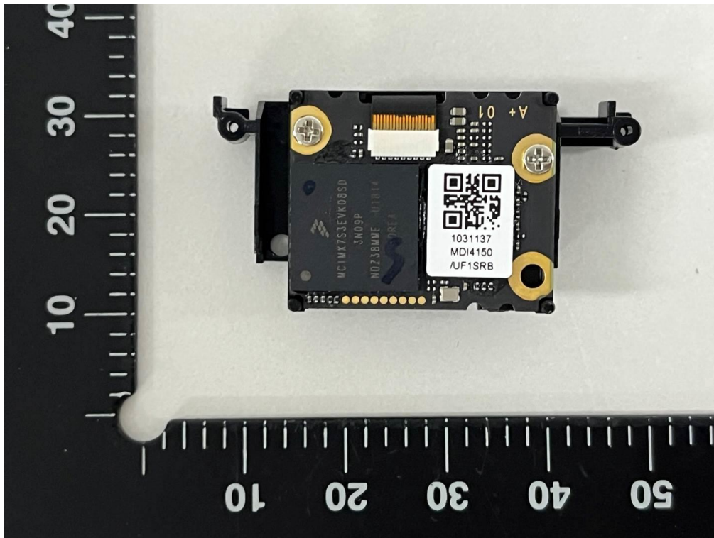
Scanner (rear)
