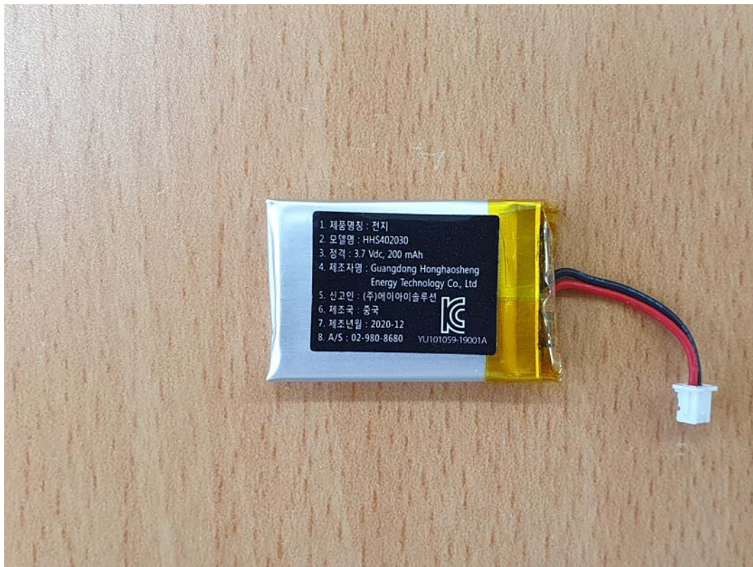
Battery - Front
