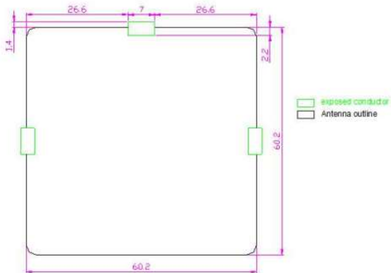
Figure F-1 Antenna Location
