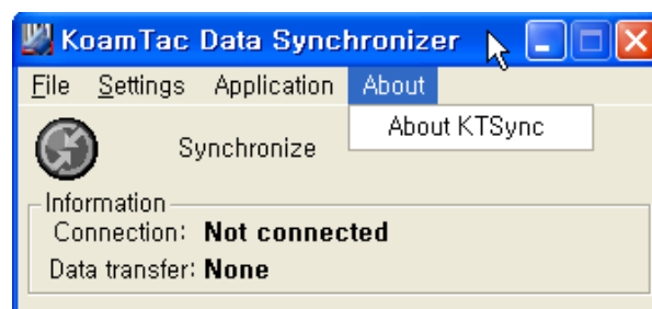
Figure 20 - About Menu
