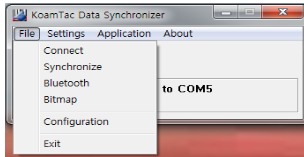
Figure 17 - File Menu
