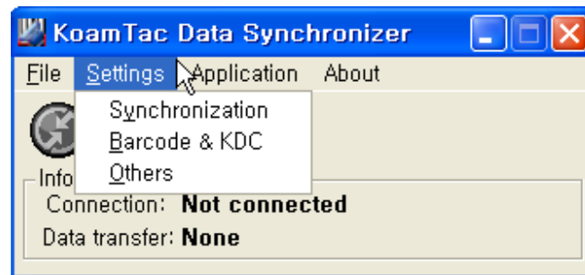
Figure 18 – Setting Menu
