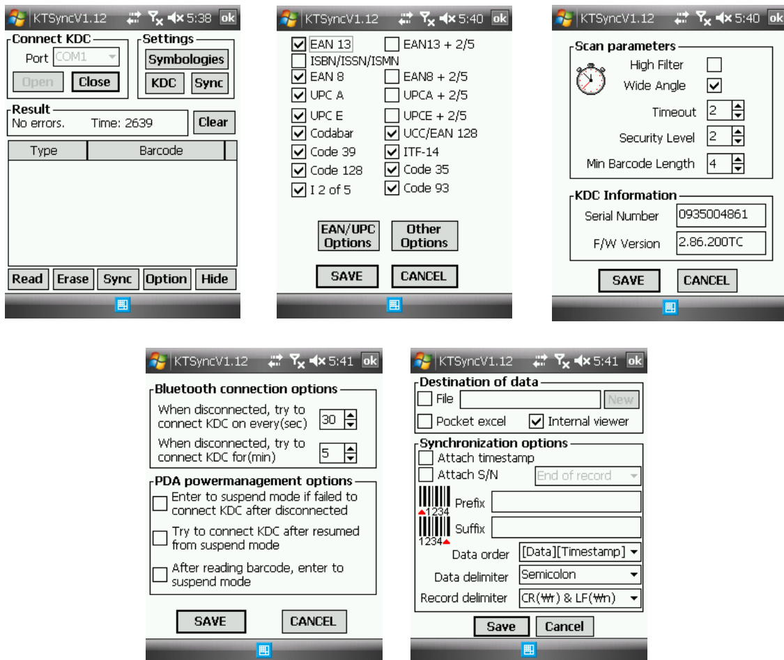
Figure 28 - Mobile pKTSync
