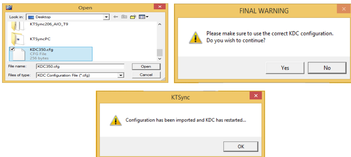
Figure 23 – Configuration
