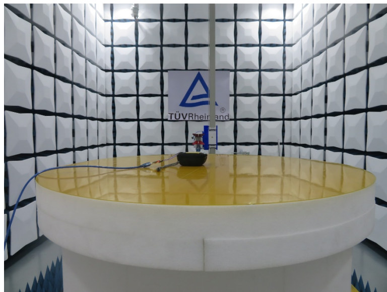
Photograph 2: Set-up for Radiated Spurious Emission, Above 1GHz
