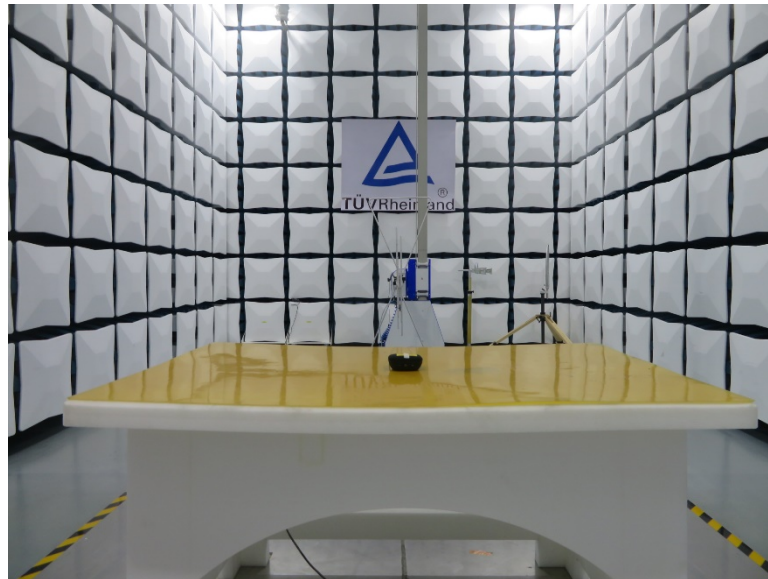
Photograph 1: Set-up for Radiated Spurious Emission, Below 1GHz
