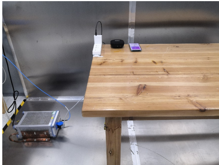
Photograph 3: Set-up for Conducted Emission on AC Mains
