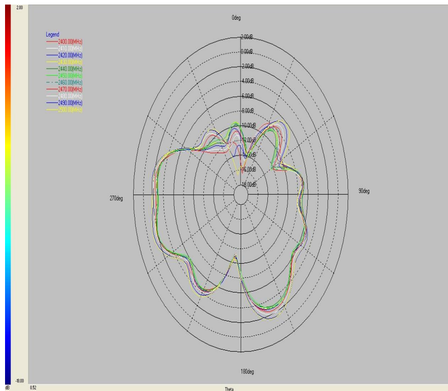
PHI 0 degree
