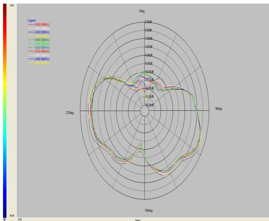
PHI 90 degree
