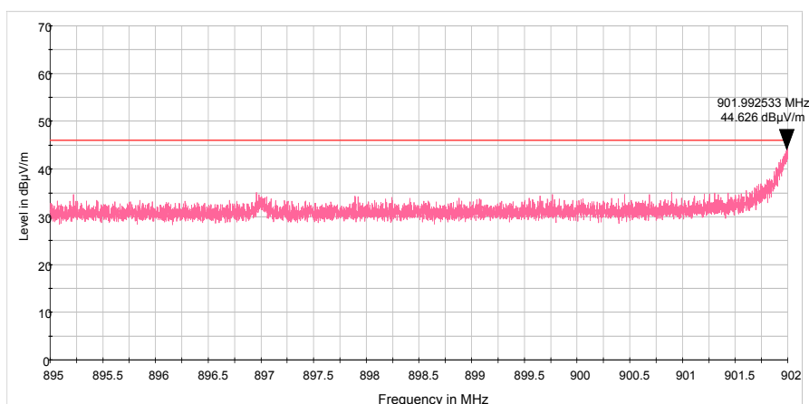
Plot 7.3.4 High band edge emission test result
