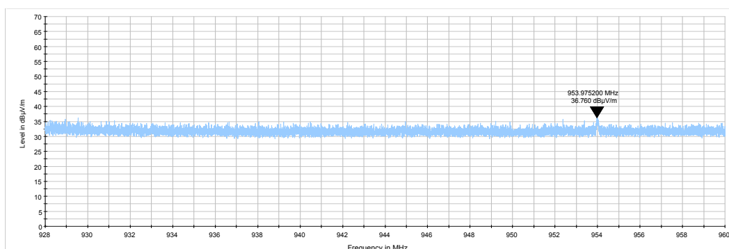
Plot 7.3.10 Radiated emission measurements from 928 to 960 MHz at the high carrier frequency
