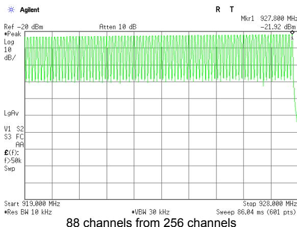
Plot 7.5.2 Number of hopping frequencies GFSK
