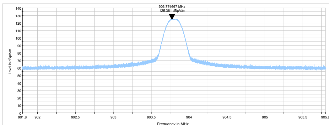
Plot 7.2.11 Field strength of carrier at mid frequency GFSK 50 kbps
