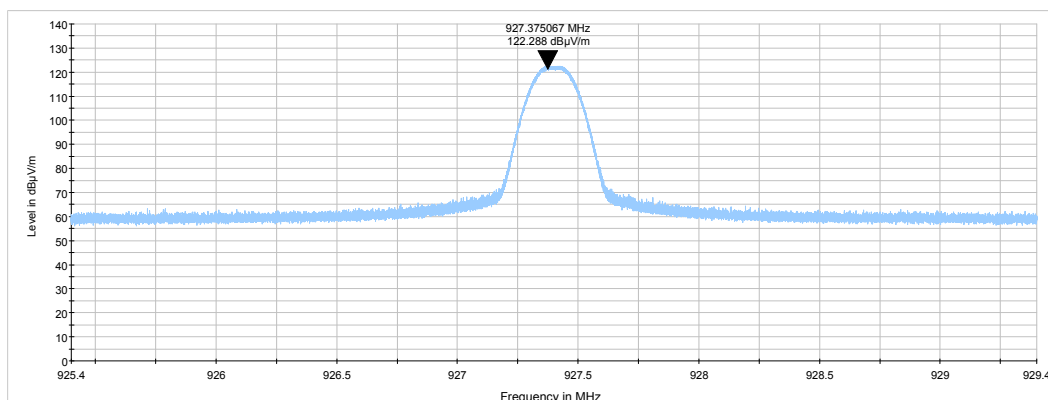
Plot 7.2.12 Field strength of carrier at high frequency GFSK 50 kbps
