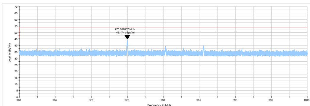
Plot 7.3.12 Radiated emission measurements from 960-1000 MHz at the mid carrier frequency
