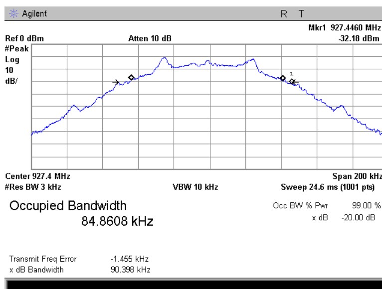
Plot 7.1.12 The 20 dB bandwidth test result at high frequency with GFSK 50.0 kbps
