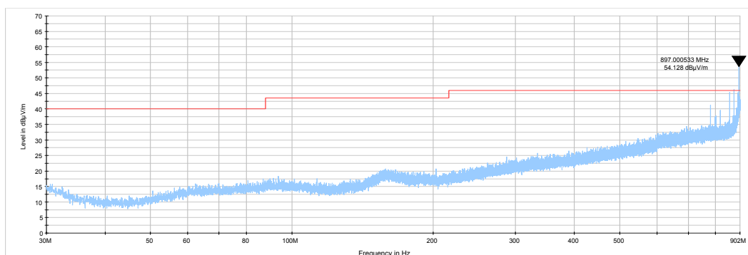
Plot 7.3.7 Radiated emission measurements from 30 to 902 MHz at the high carrier frequency
