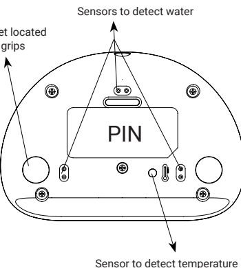
Water Detector-Back view
