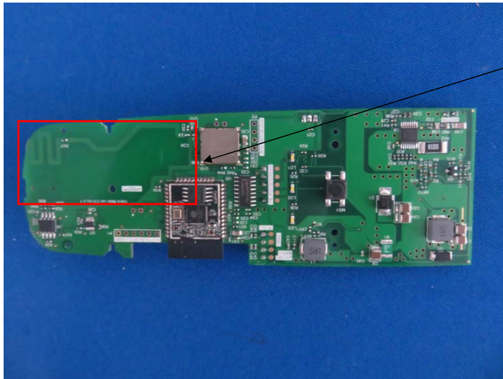
915MHz Antenna
