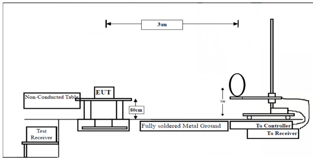
Figure 1. Below 30MHz
