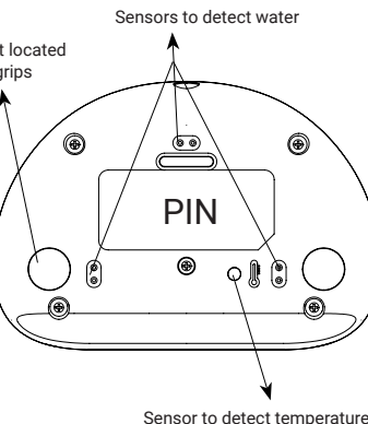
Water Detector-Back view
