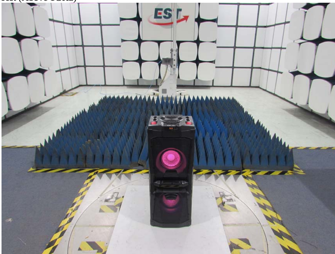
Radiated Test (Above 1GHz)
