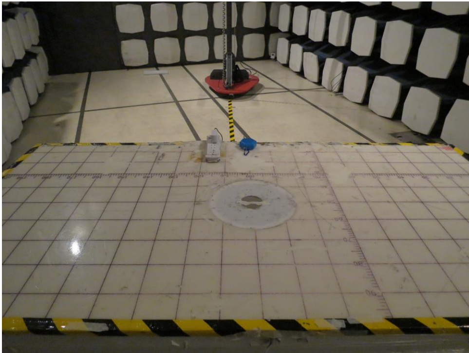
Front View of Radiated Emission up to 1GHz
