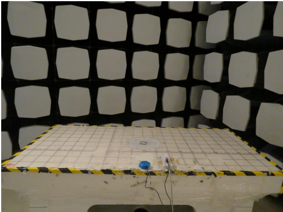
Back View of Radiated Emission up to 1GHz
