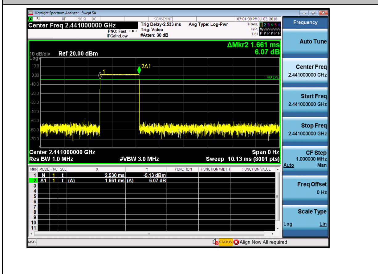
Dwell Time_DH3_2441
