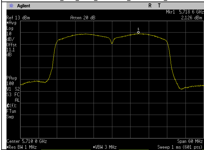
5710MHz_Ch_142_40MHz_n-mode Ant C
