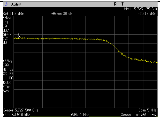
5725-5730MHz_Ch142_40MHz_n-mode Ant B
