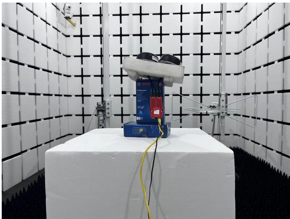
EIRP Output Power
