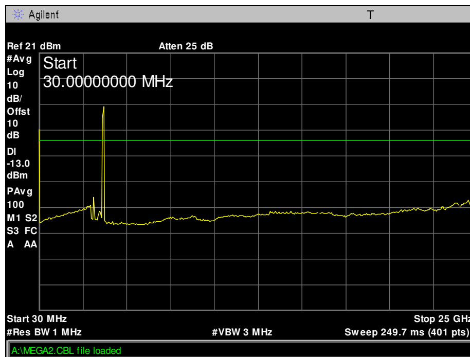
Plot 53. Conducted Spurious Emissions - High - 3688.4MHz - BW20MHz - Chain0
