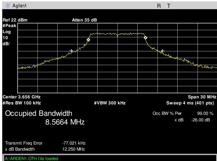
Plot 31. Occupied Bandwidth - Low - 3655.9MHz - BW10MHz - Chain0
