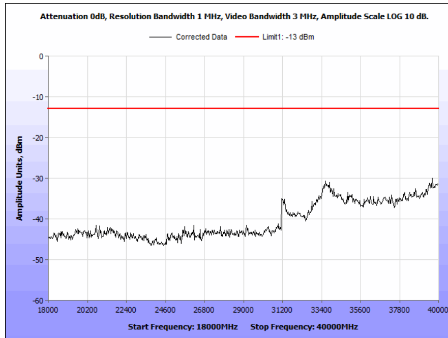
Plot 69. Spurious TX Emissions 20 MHz BW, High Channel 18GHz - 40GHz
