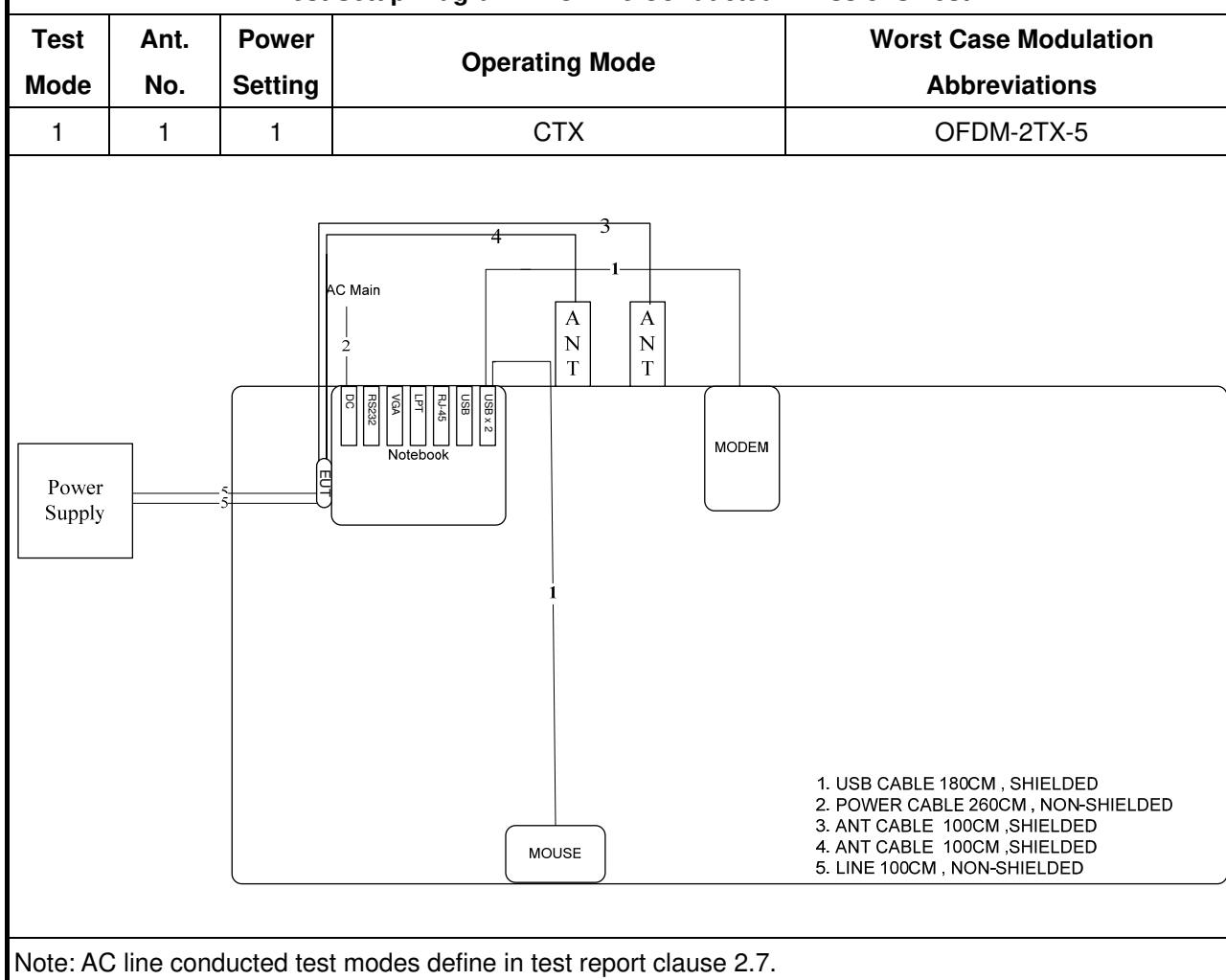
Test Setup Diagram - AC Line Conducted Emissions Test
