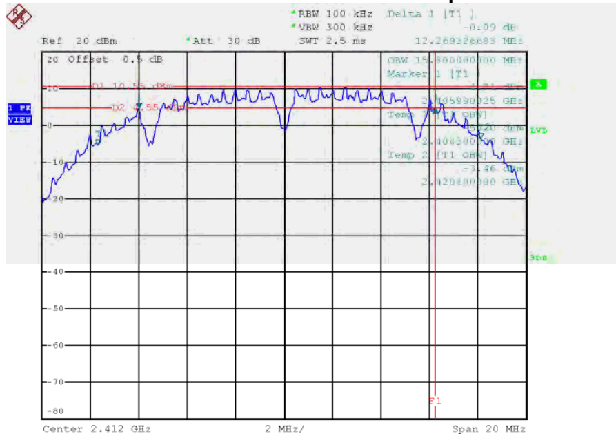
IEEE 802.11b/2412 MHz/6 dB and 99% Occupied Bandwidth
