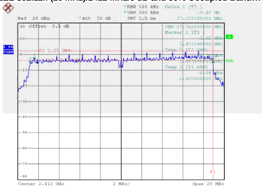
IEEE 802.11n (20 MHz)/2412 MHz/6 dB and 99% Occupied Bandwidth
